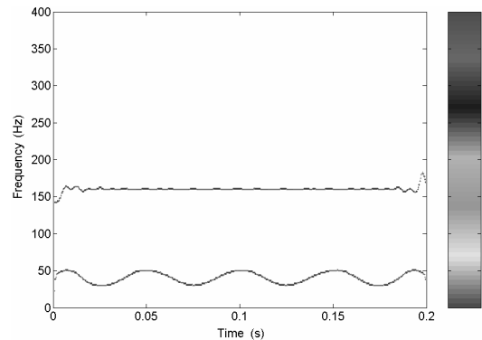
Fig. 4. THT spectrum of multi-components signal (contour plot).
